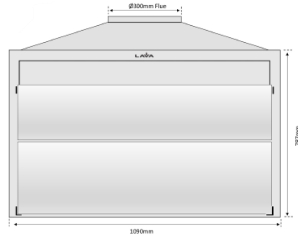
WOOD BURNING BRAAI STAINLESS STEEL FACE AND MILD STEEL INTERNAL
